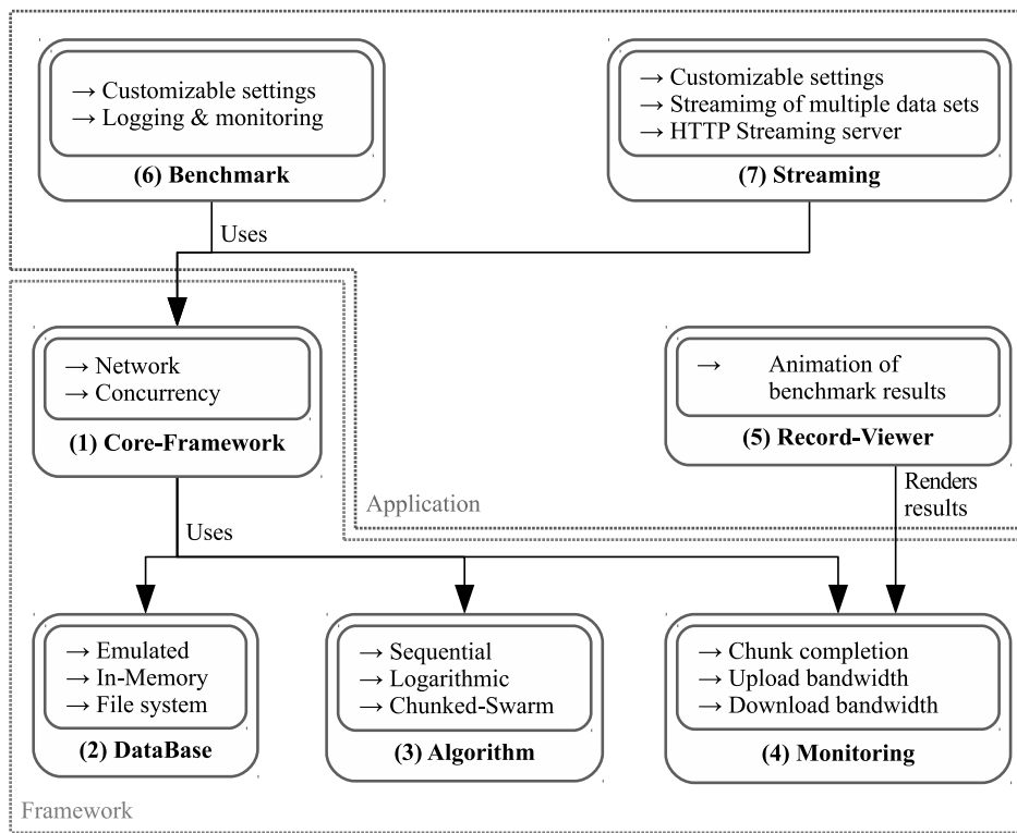
Figure 3.1.: Software Architecture
