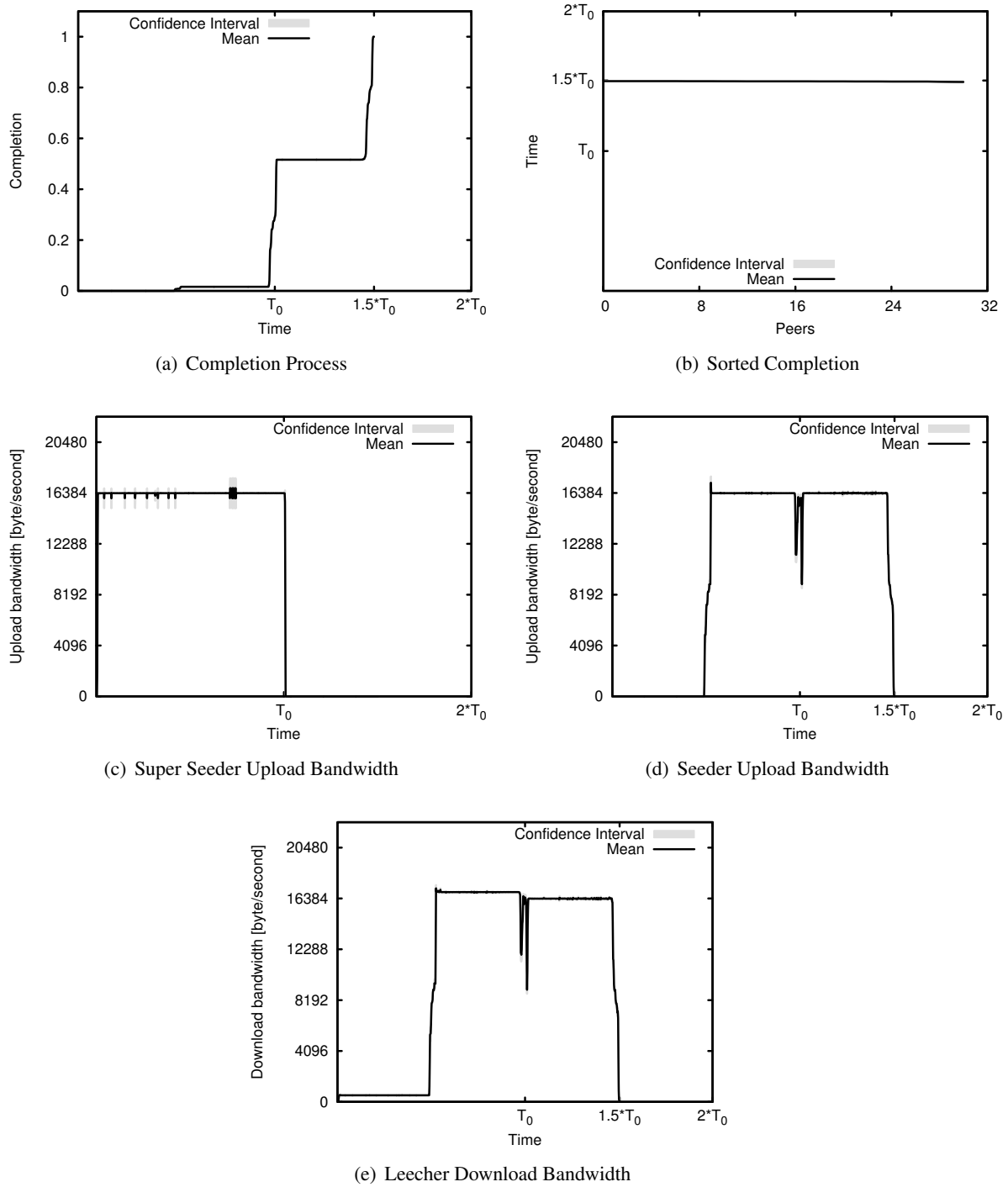
Figure 5.4.: Scenario 4 - 32 Peers
